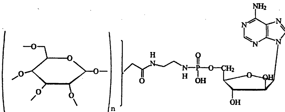
Figure 1C. Dextran-CM-EDA-P-araA
